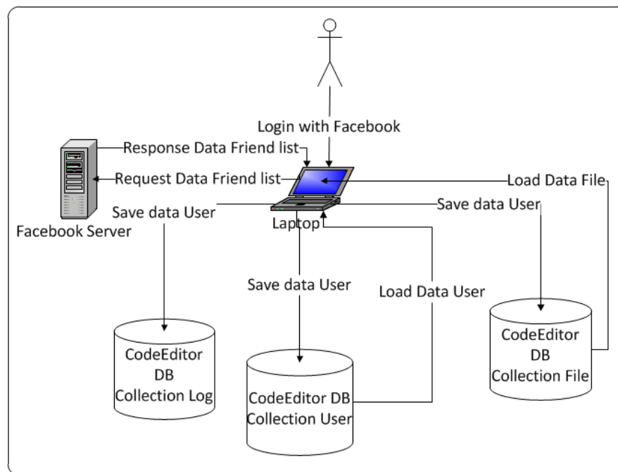
Fig. 7. Login Architecture
