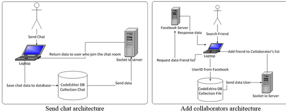
Fig. 8. Chat and add collaborator architecture
