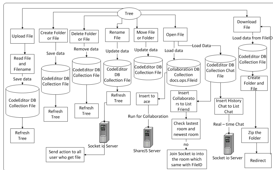
Fig. 9. Tree project folder and file architecture
